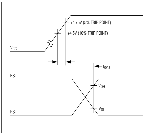
Figure 8. VCC Detect Reset Output Delay (Power-Up)
