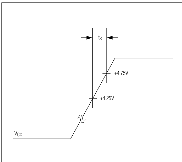
Figure 6. Power-Up Slew Rate
