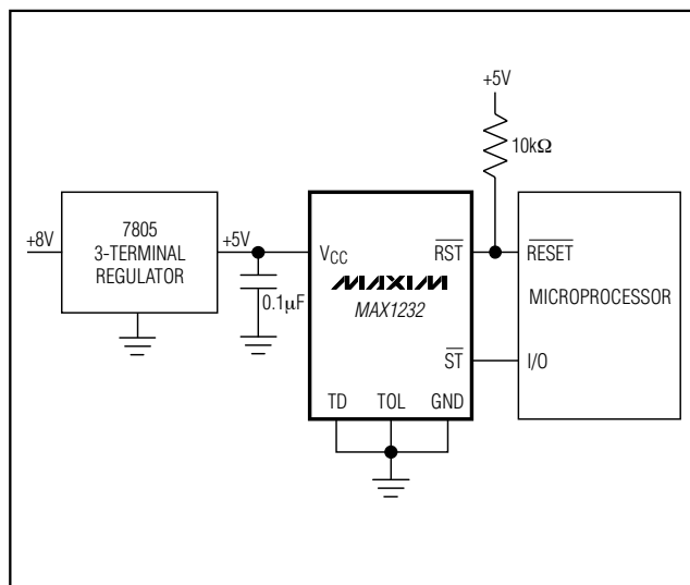
Figure 2. Watchdog Timer
