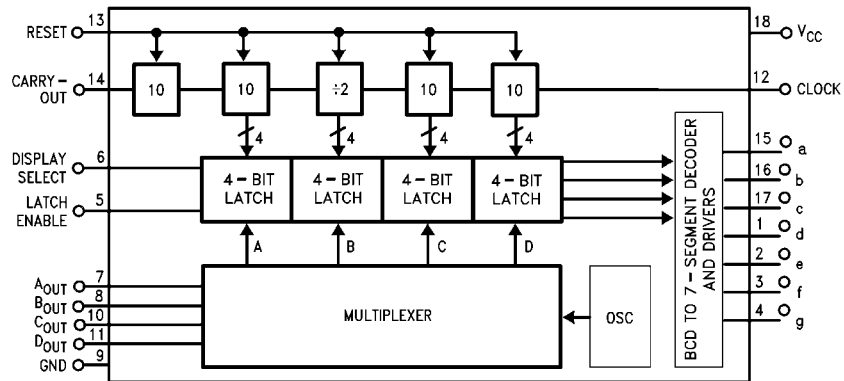
MM74C928
