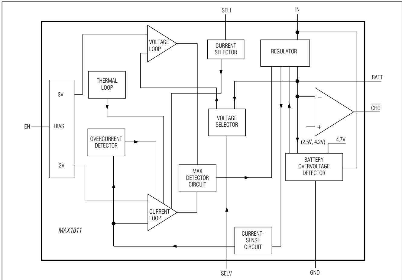
Figure 1. Functional Diagram
