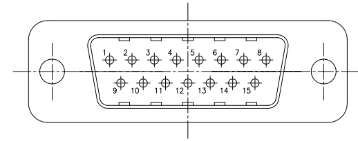
15 SIZE PIN
