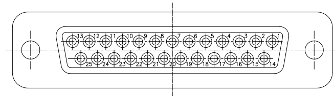
25 SIZE SOCKET
