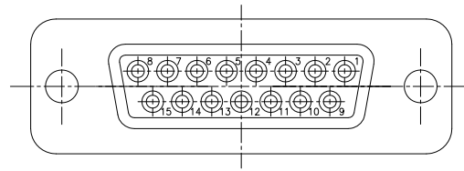
15 SIZE SOCKET
