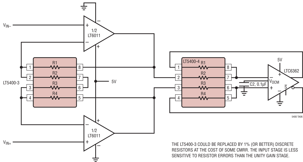
Gain of 10, 106dB CMRR, Discrete Component, Fully-Differential Instrumentation Amplifier
