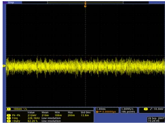
FIGURE 15. RIPPLE VOLTAGE (54 LEDs, V_{IN} = 12V , 20mA EACH, C_{OUT} = 4 \times 4.7\mu F/50V )
