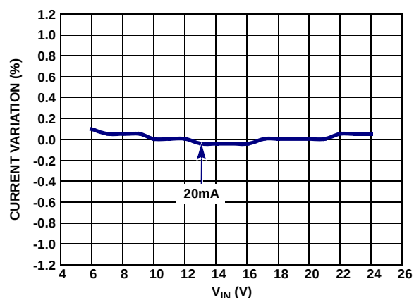
FIGURE 5. CURRENT REGULATION
