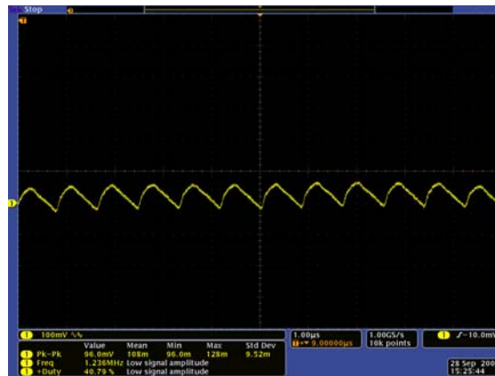
FIGURE 16. RIPPLE VOLTAGE ZOOM IN (54 LEDs, V_{IN} = 12V , 20mA EACH, C_{OUT} = 4 \times 4.7\mu F/50V )
