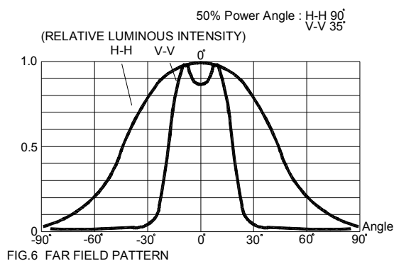
FIG.6 FAR FIELD PATTERN
