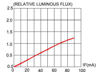
FIG.2 RELATIVE LUMINOUS FLUX VS. FORWARD CURRENT
