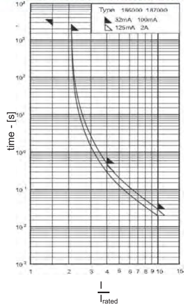
Time-Current Characteristics
