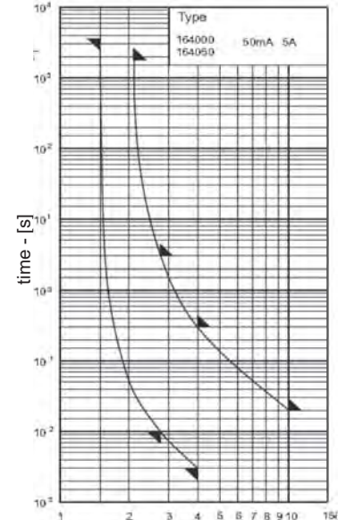
Time-Current Characteristics
