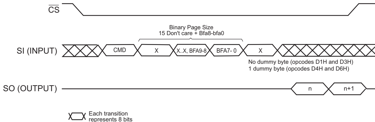
Figure 21-4. Buffer Read
