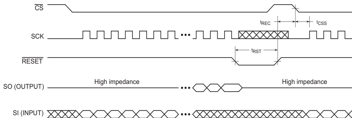
Figure 19-2. Reset Timing
