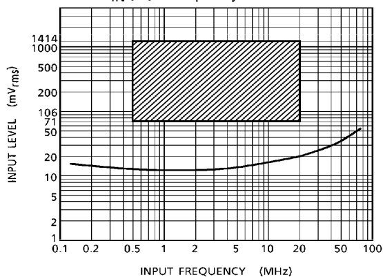
AM IN (LF) Frequency Characteristics
