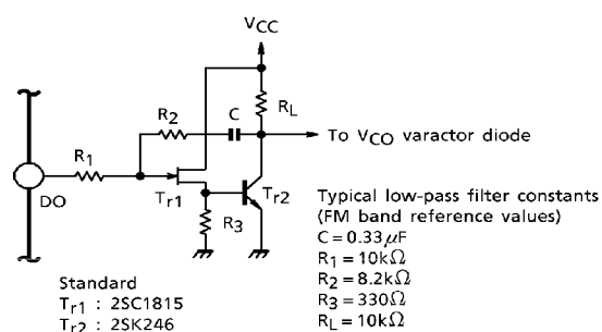
Typical Active Low-Pass Filter Circuit Fig.9
