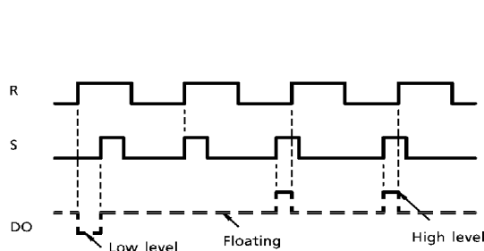
DO Output Timing Chart Fig.8
