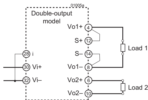
Fig. 5 Independent-output configuration
