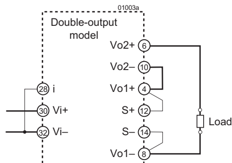
Fig. 3 Series-output configuration
