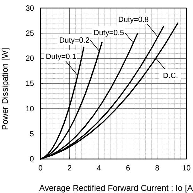
Fig.8 Io-Pf Characteristics
