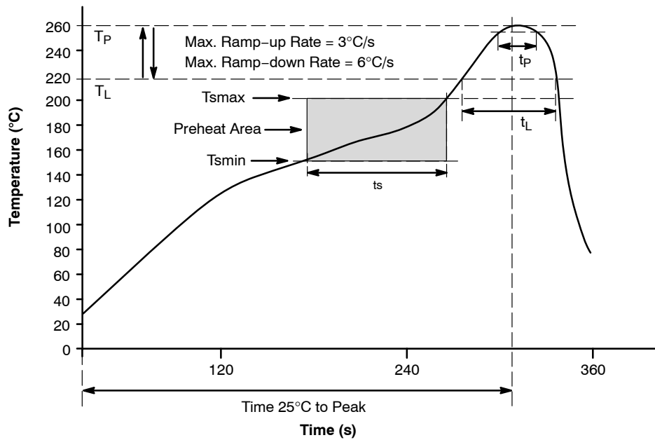
Figure 8. Reflow Profile
