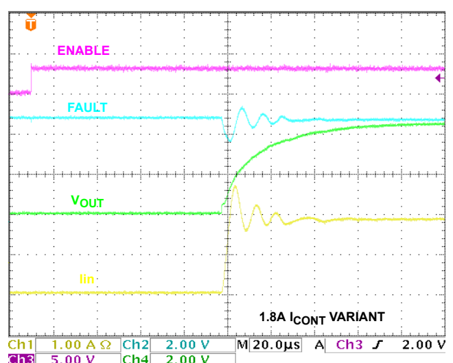
FIGURE 24. V_{IN} = 5V TURN-ON INTO 2.7Ω
