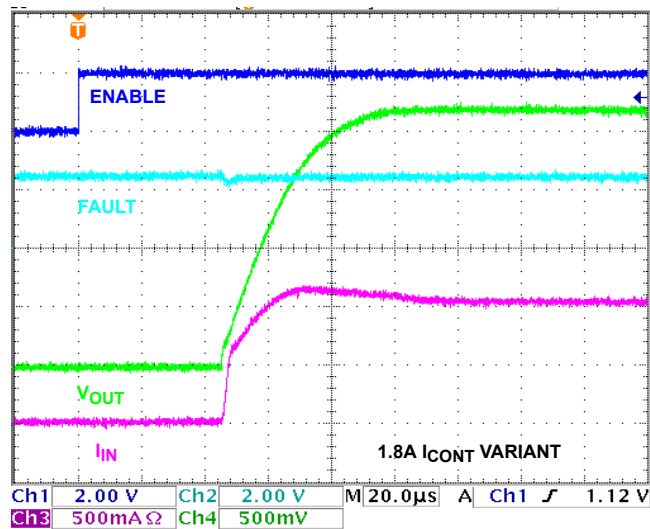
FIGURE 23. V_{IN} = 2.5V TURN-ON INTO 2.2Ω
