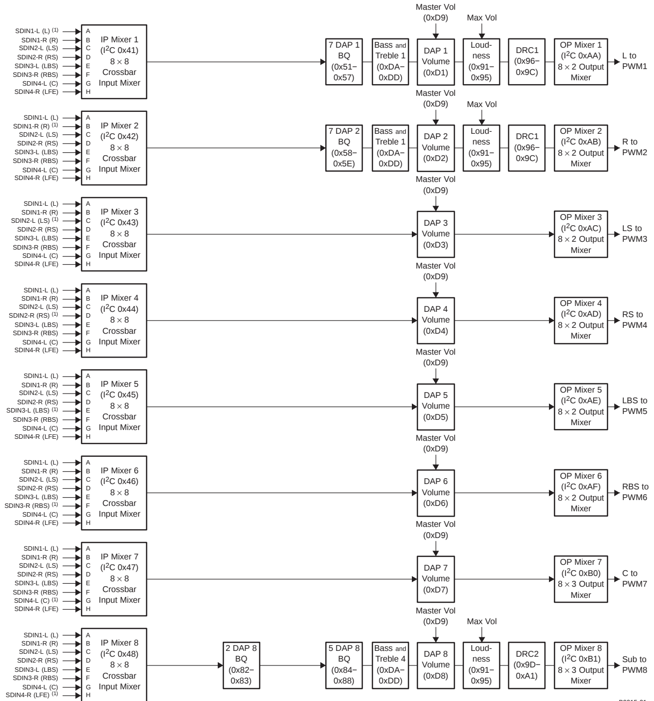
Figure 2-2. TAS5518C Architecture With I²C Registers ( f_s = 176.4 kHz or f_s = 192 kHz)
