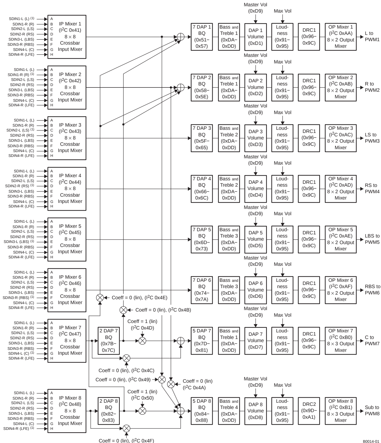
Figure 2-1. TAS5518C DAP Architecture With I²C Registers ( f_s \leq 96 kHz)
