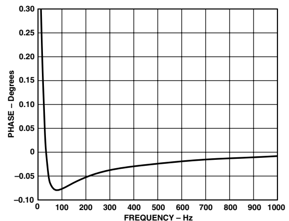
Figure 10. Phase Error Between Channels (0 Hz to 1 kHz)
