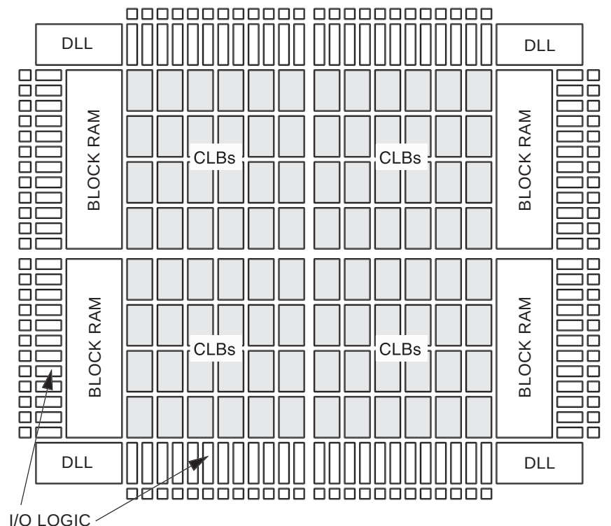
Figure 1: Basic Spartan-IIE Family FPGA Block Diagram
