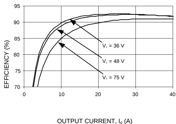
Figure 8. Converter Efficiency Vs Load at Room temperature.
