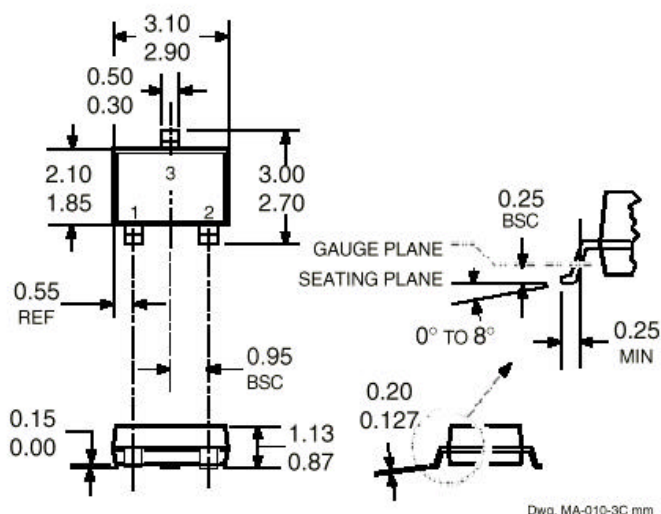
Dimensions in Millimeters (controlling dimensions)
