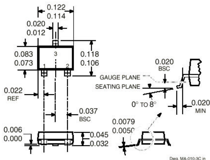
Dimensions in Inches (for reference only)
