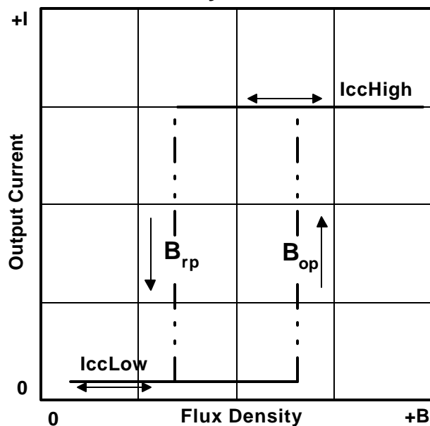
A1181/3/4 Hysteresis Curve
