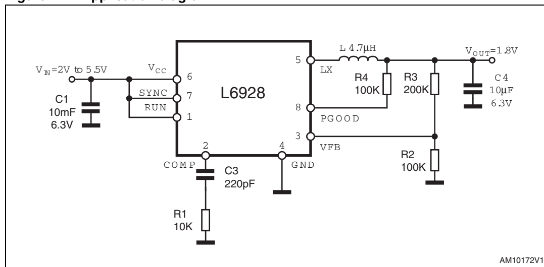
Figure 1. Application diagram
