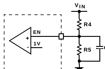
FIGURE 38. EXTERNAL RESISTOR DIVIDER
