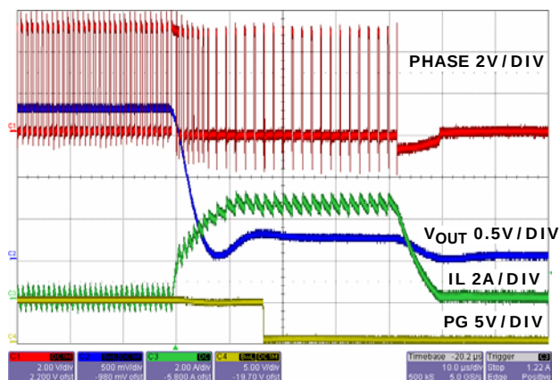
FIGURE 33. OUTPUT SHORT CIRCUIT
