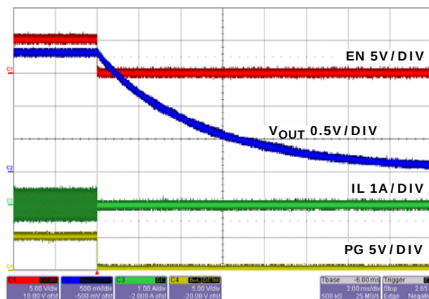
FIGURE 28. SOFT-DISCHARGE SHUTDOWN
