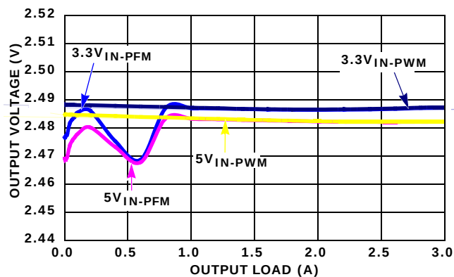
FIGURE 13. V_{\text{OUT}} REGULATION vs LOAD (1MHz, V_{\text{OUT}} = 2.5\text{V} )
