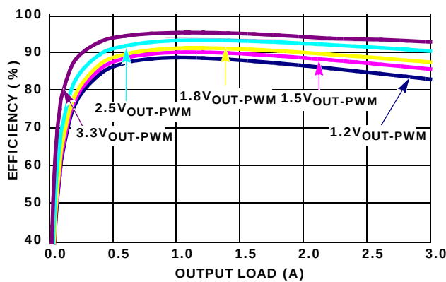
FIGURE 5. EFFICIENCY vs LOAD (1MHz 5 V_{\text{IN}} PWM)
