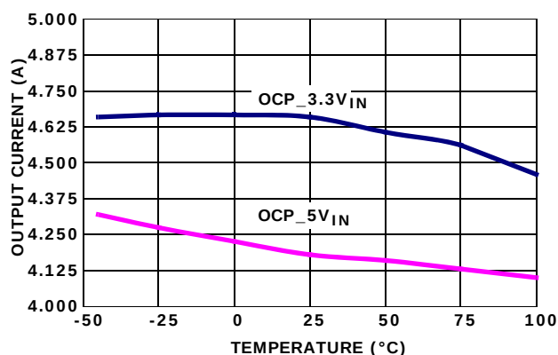
FIGURE 35. OUTPUT CURRENT LIMIT vs TEMPERATURE
