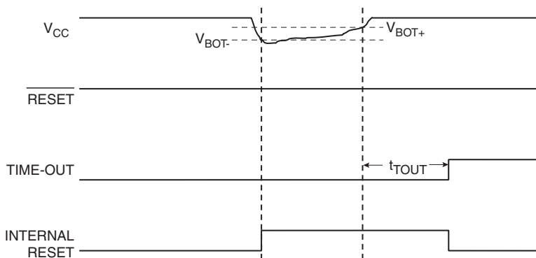
Figure 9-3. Brown-out Reset During Operation
