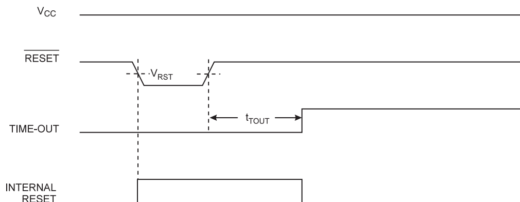
Figure 9-2. External Reset During Operation
