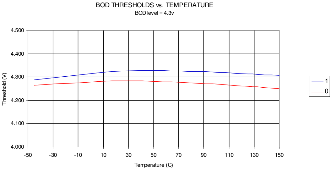
Figure 27-21. BOD Thresholds vs. Temperature (BOD level is 4.3V)
