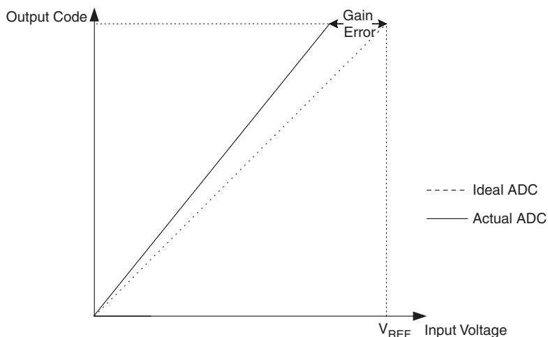
Figure 21-11. Gain Error
