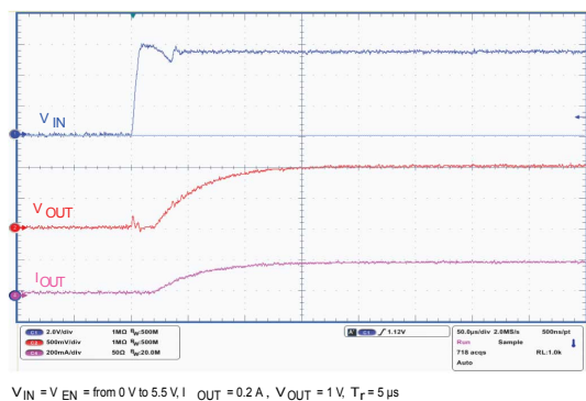
Figure 20. Turn-on time ( V_{OUT} = 1\text{ V} )
