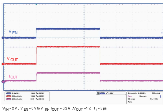
Figure 18. Enable startup ( V_{OUT} = 1\text{ V} )
