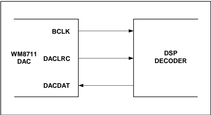
Figure 18 Master Mode
