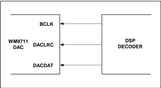
Figure 19 Slave Mode
