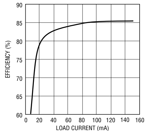
Efficiency Curve
