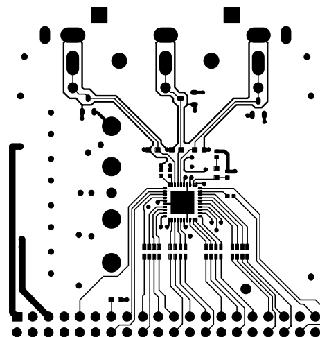
Figure 26: EVAL-ADV7392/93EBZ Layer 1
