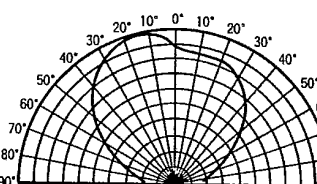
Directive Characteristics
