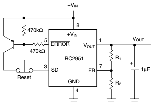
Figure 8. Latch Off When Error Flag Occurs
