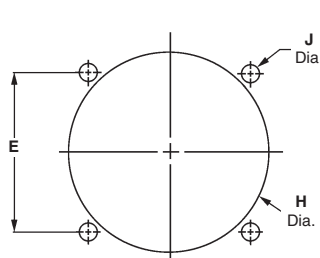
Rear Mount Panel Cutout
