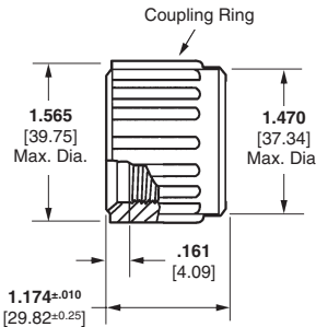
Coupling Ring
