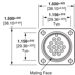
Mating Face
