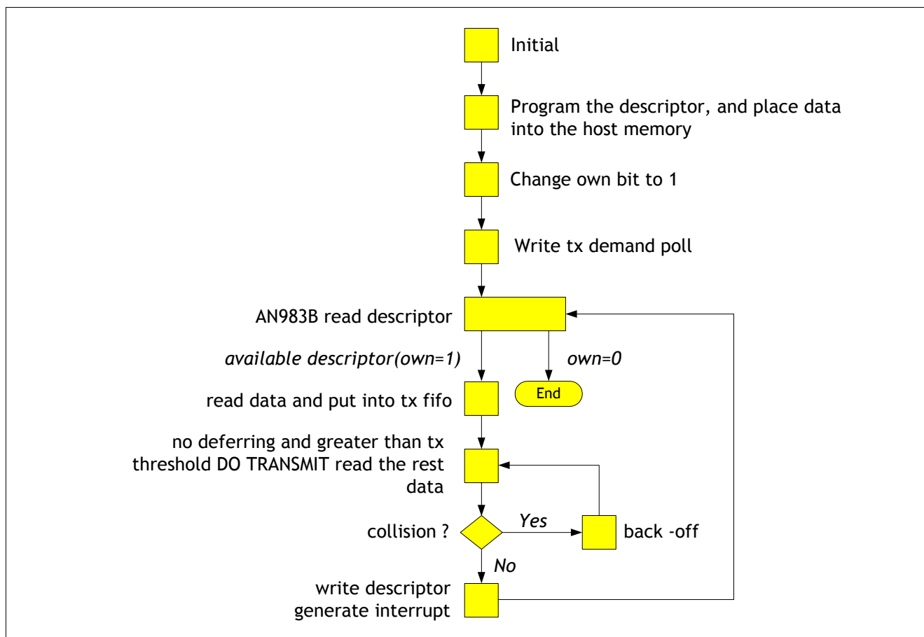
Figure 9 Transmit Flow
