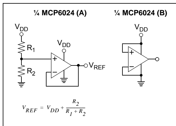
FIGURE 4-11: Unused Operational Amplifiers.
