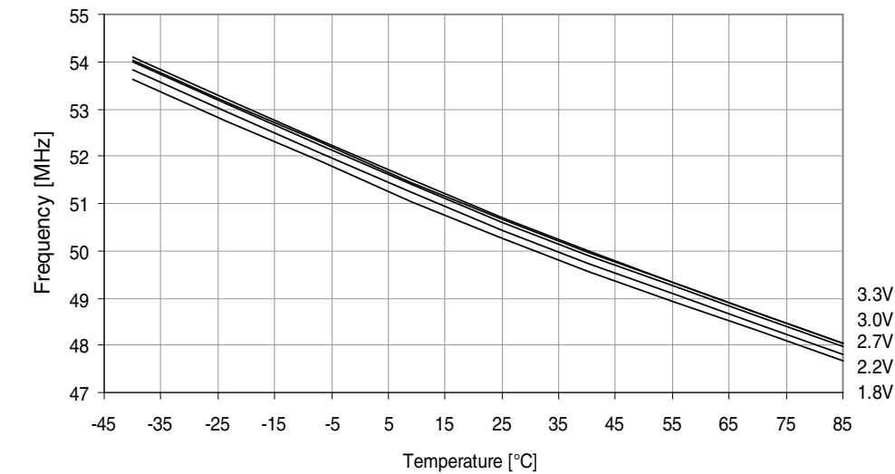
Figure 37-244. 48MHz internal oscillator frequency vs. temperature. DPLL disabled.
