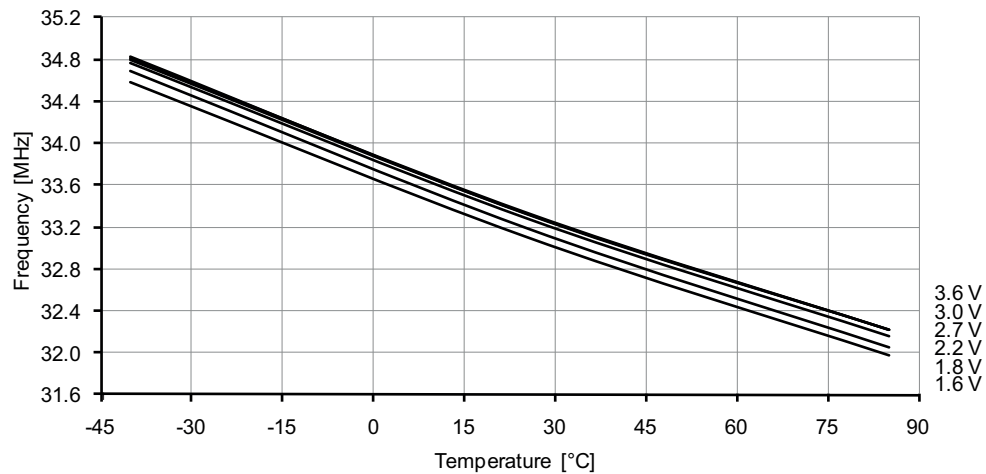
Figure 37-157. 32MHz internal oscillator frequency vs. temperature. DFLL disabled.
