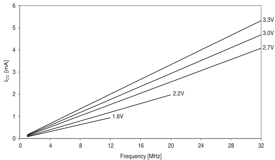
Figure 37-175. Idle mode supply current vs. frequency.
