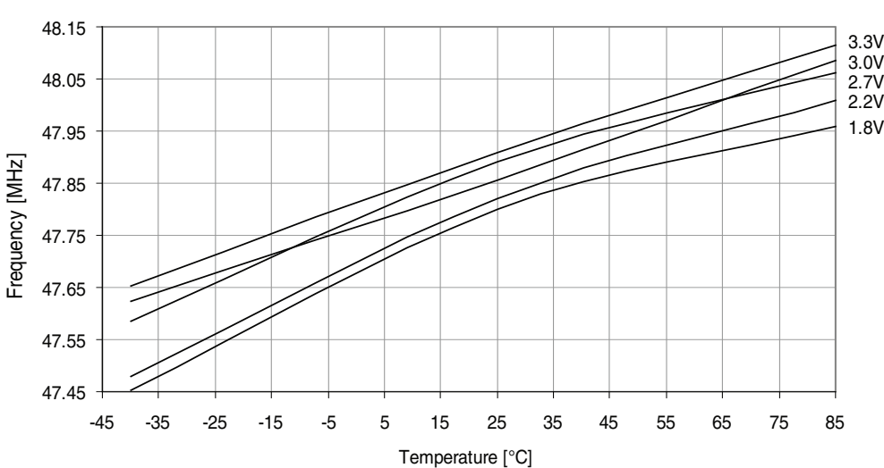
Figure 37-245. 48MHz internal oscillator frequency vs. temperature. DPLL enabled, from the 32.768kHz internal oscillator.
