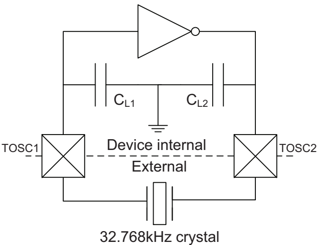
Figure 36-4. TOSC input capacitance.
