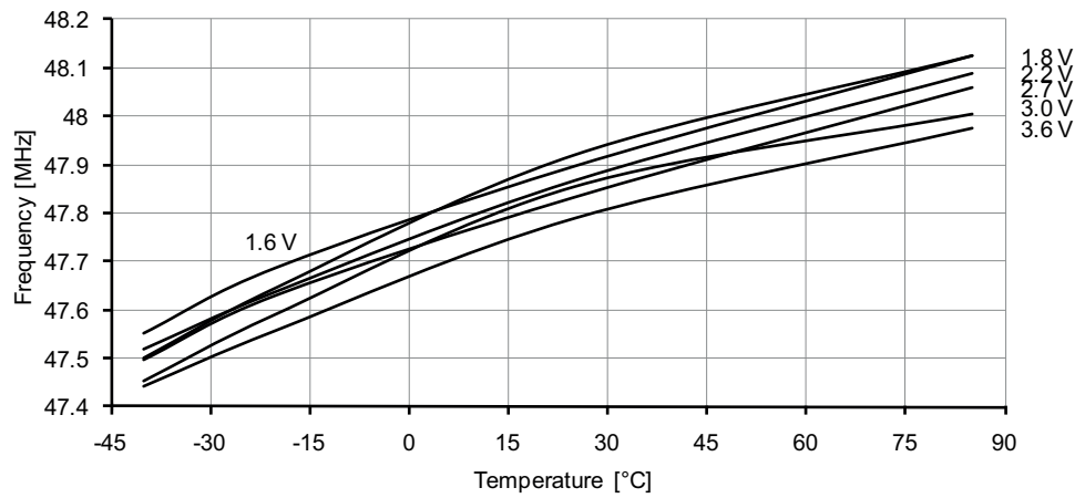
Figure 37-162. 48MHz internal oscillator frequency vs. temperature. DFLL enabled, from the 32.768kHz internal oscillator.
