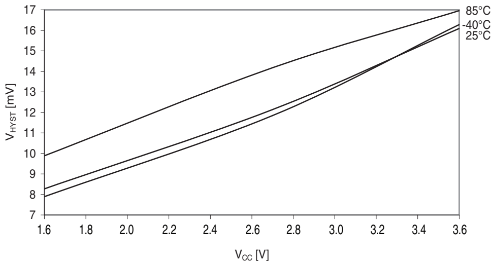
Figure 37-300. Analog comparator hysteresis vs. V_{CC} . High-speed, small hysteresis.
