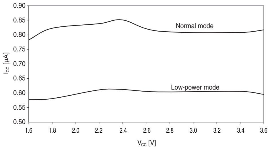
Figure 37-266. Power-save mode supply current vs. V_{CC} .
