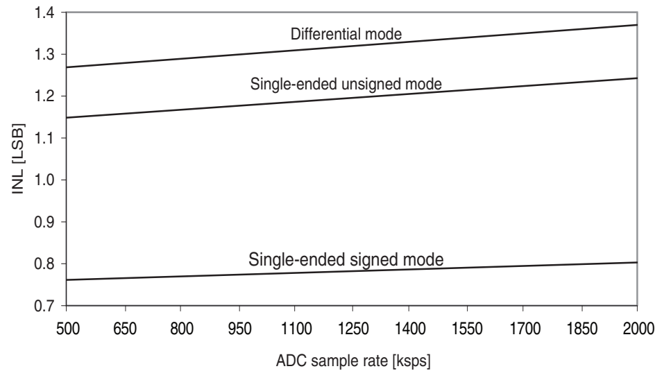
Figure 37-202. INL error vs. sample rate. T = 25\text{ }^{\circ}\text{C} , V_{CC} = 3.6\text{V} , V_{REF} = 3.0\text{V} external.
