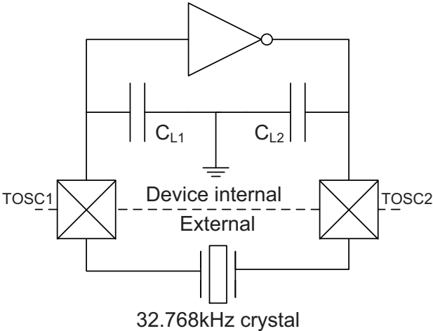
Figure 36-18.TOSC input capacitance.
