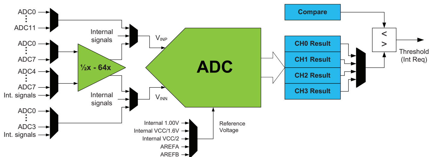
Figure 28-1. ADC overview.
