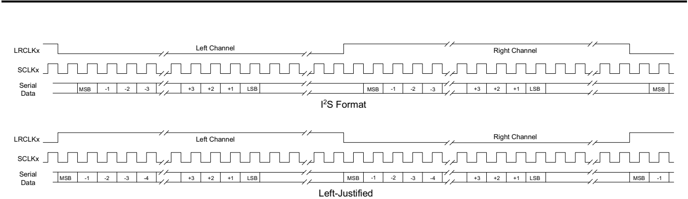
FIGURE 8. SAI PORT SUPPORTED DATA FORMATS FOR DELIVERY OF LINEAR PCM OR COMPRESSED AUDIO DATA
