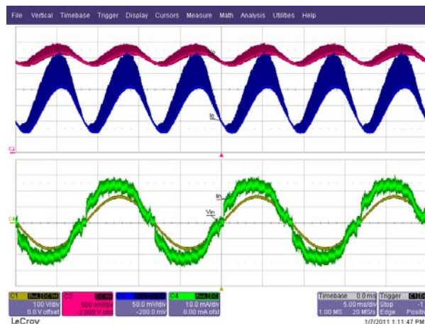
Figure 44 – 115 VAC / 60 Hz.
