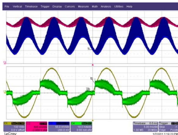
Figure 46 – 265 VAC / 63 Hz.
