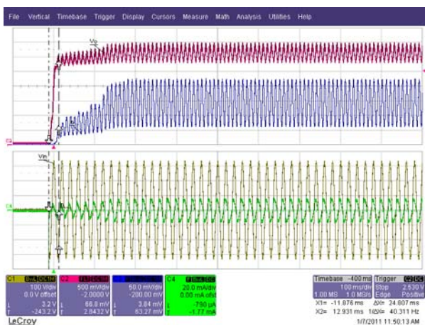
Figure 41 – 230 VAC / 50 Hz.
