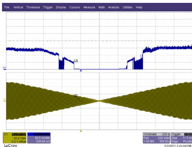
Figure 65 – 90-0-90 VAC / 50 Hz at 0.1 \text{ V / s} Slew Rate. LED = 3 V / 366 mA. Ch1(Yellow): V_{IN} , 50 V / div. Ch3(Blue): I_O , 100 mA / div. Time Scale: 200 s / div.
