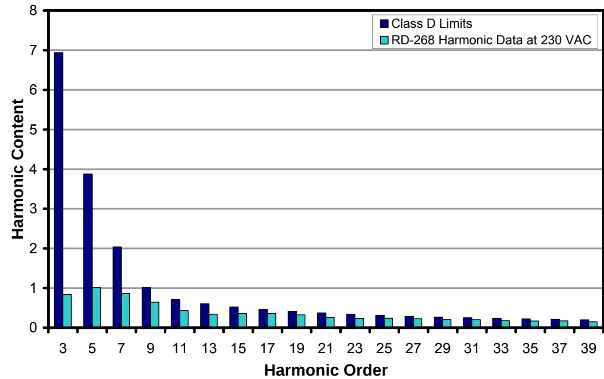
Figure 15 – 230 V UUT Harmonic Content.
