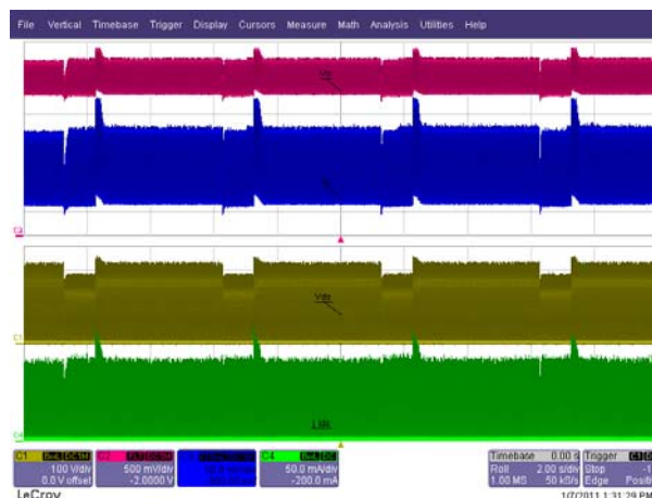
Figure 48 – 115-85-115 VAC / 60 Hz.
