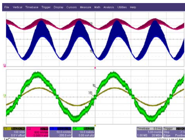
Figure 43 – 90 VAC / 47 Hz.
