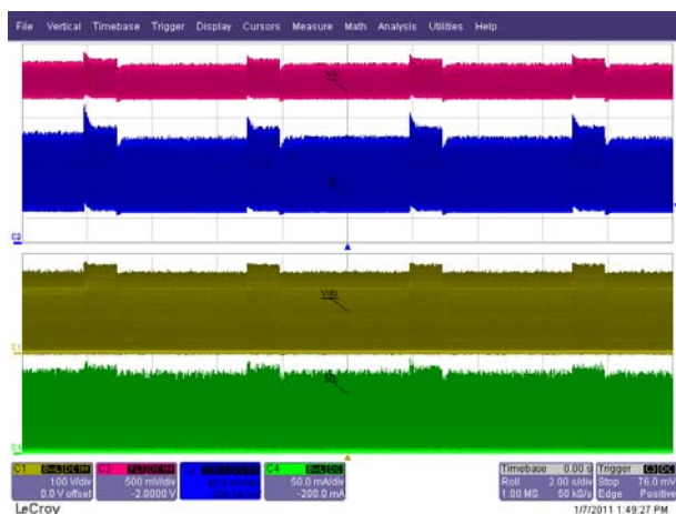
Figure 53 – 115-132-115 VAC / 60 Hz. LED = 3 V / 366 mA. Ch1(Yellow): V_{DS} , 100 V / div. Ch2(Red): V_{IN} , 0.5 V / div. Ch3(Blue): I_O , 100 mA / div. Ch4(Green): I_{DS} , 50 mA / div., 2 s / div.
