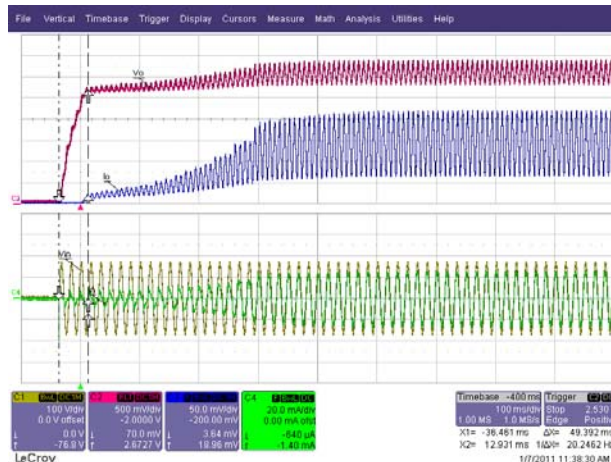
Figure 40 – 115 VAC / 60 Hz.
