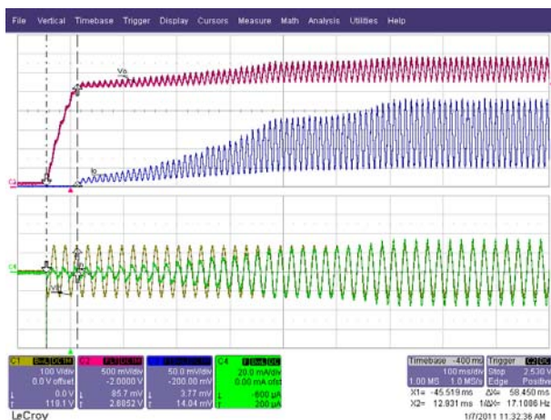
Figure 39 – 90 VAC / 47 Hz.
