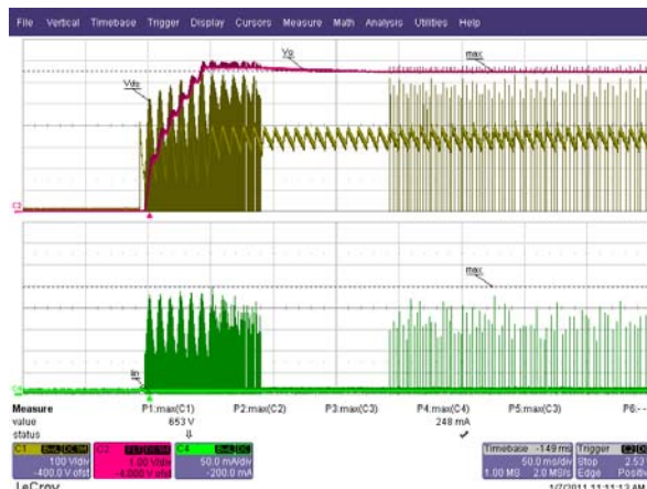
Figure 38 – 265 VAC. Load Open. Ch1(Yellow): V_{DS} , 100 V / div. Ch2(Red): V_O , 1 V / div. Ch4(Green): I_{DS} , 50 mA / div., 50 ms / div.
