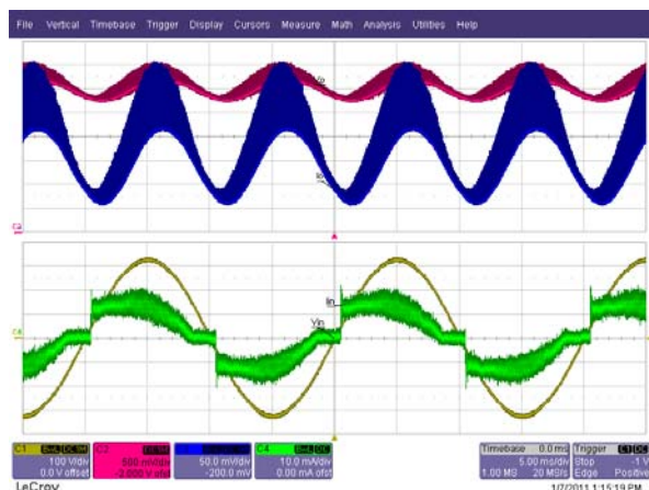
Figure 45 – 230 VAC / 50 Hz.
