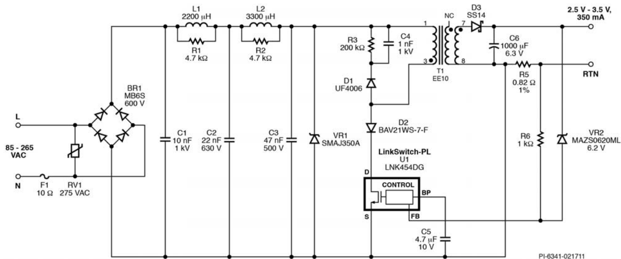
Figure 5 – Schematic.
