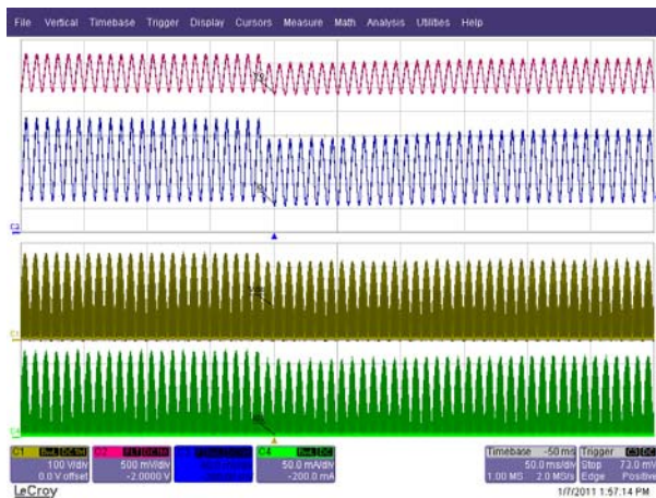
Figure 55 – 115-132-115 VAC / 60 Hz. LED = 3 V / 366 mA. Ch1(Yellow): V_{DS} , 100 V / div. Ch2(Red): V_{IN} , 0.5 V / div. Ch3(Blue): I_O , 100 mA / div. Ch4(Green): I_{DS} , 50 mA / div., 50 ms / div.
