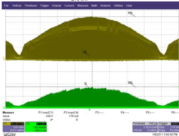
Figure 27 – 115 VAC / 60 Hz, LED = 3 V / 366 mA. Upper: V_{DRAIN} , 100 V / div., 1 ms / div. Lower: I_{DRAIN} , 0.1 A / div.
