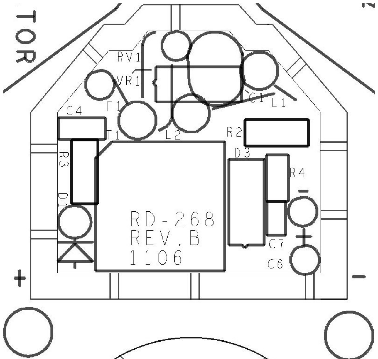
Figure 9 – Top Silkscreen.
