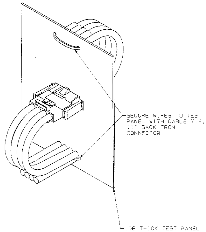
Figure 5A Vibration & Mechanical Shock Mounting Fixture Panel Mounted Samples
