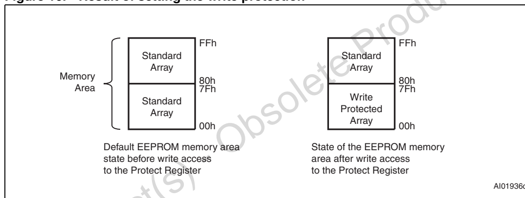
Figure 10. Result of setting the write protection
