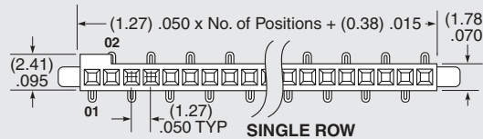
SINGLE ROW
