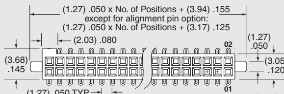
DOUBLE ROW
