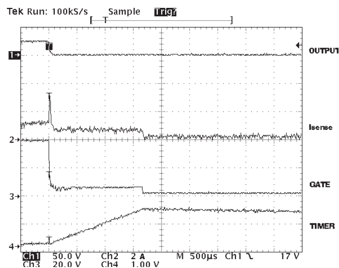
Figure 9. Short-Circuit Waveforms
