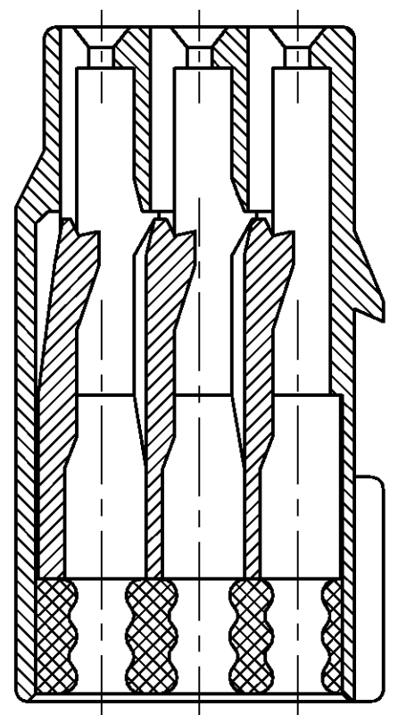
SECT. A-A
