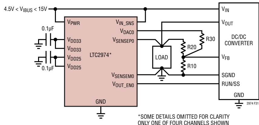
Figure 31. Application Circuit for DC/DC Converters with External Feedback Resistors
