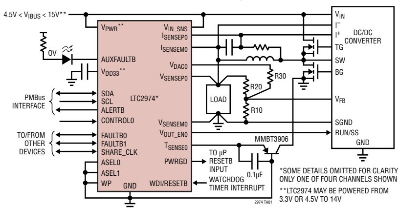
4-Channel PMBus Power System Manager
