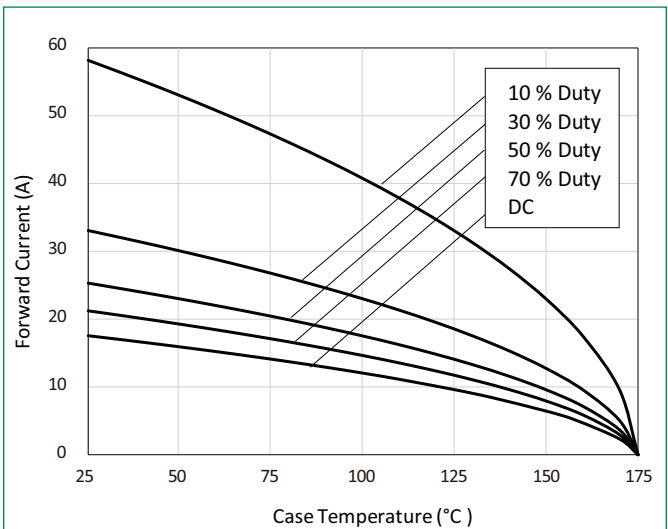
Figure 4: Current Derating (Per Leg)
