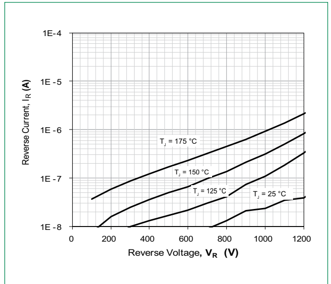
Figure 2: Typical Reverse Characteristics (Per Leg)
