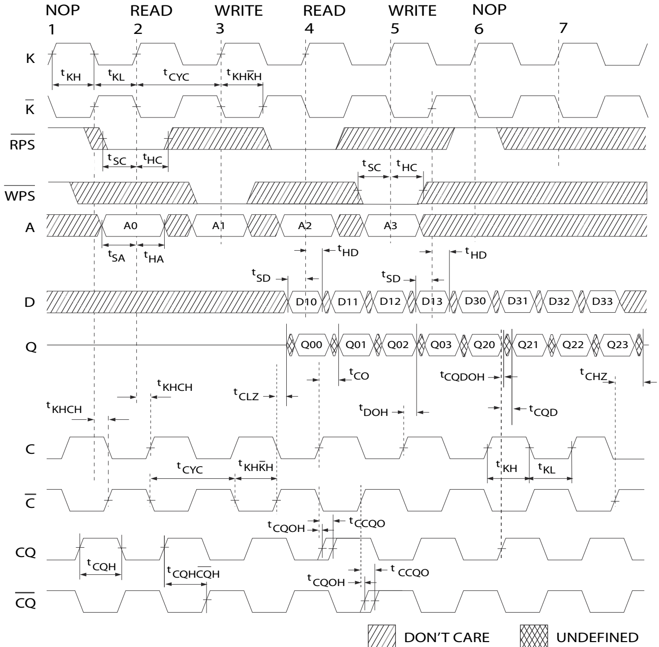
Figure 6. Read/Write/Deselect Sequence [39, 40, 41]
