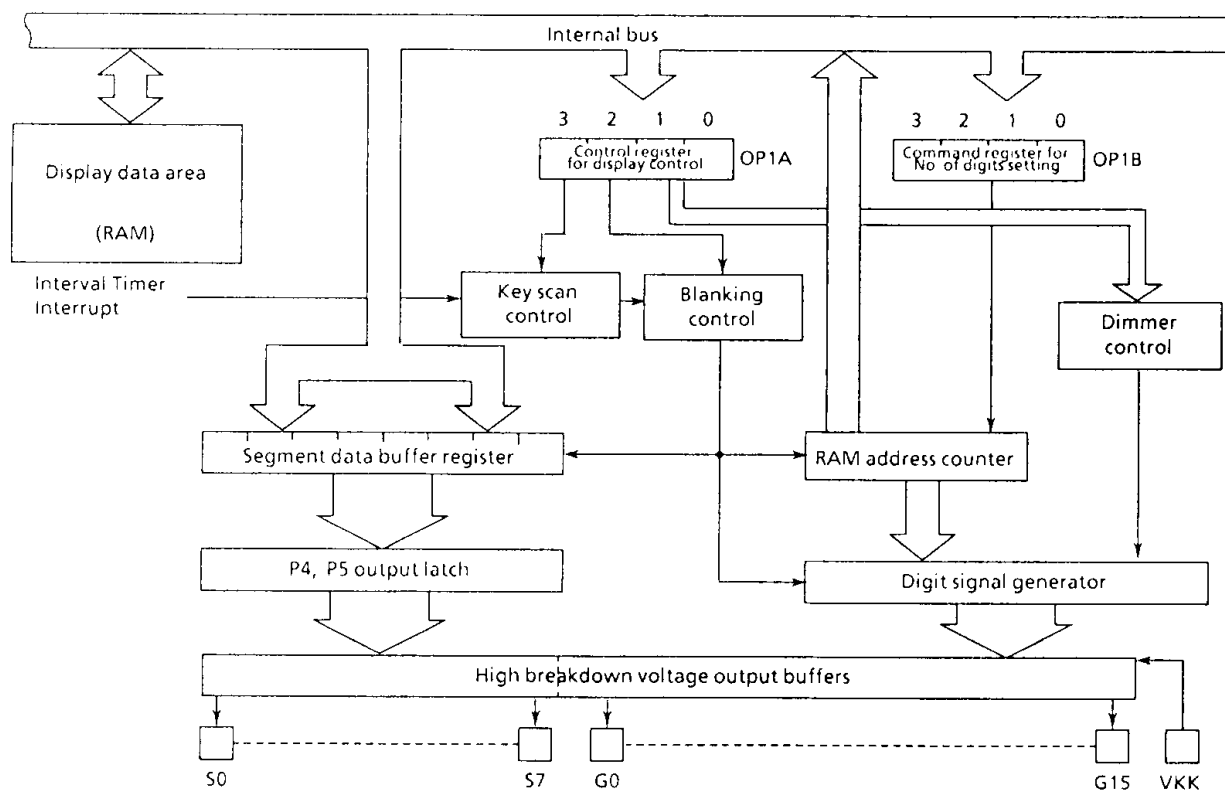
Figure 2-10. VFT driver
