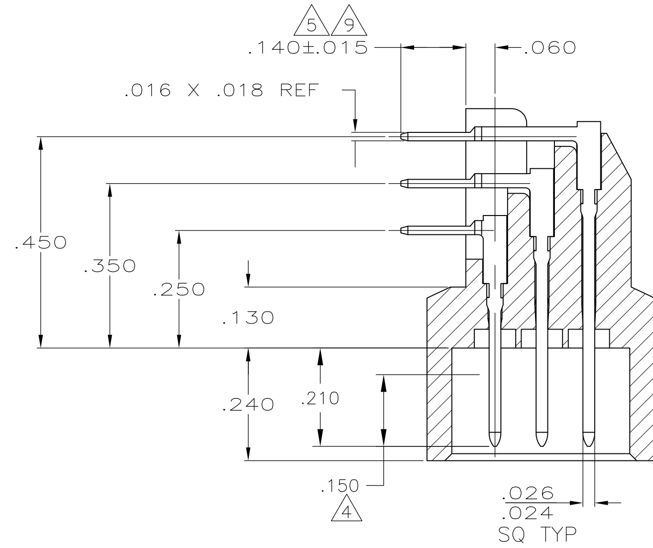
SECTION X-X
