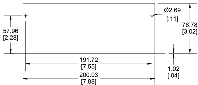
Side View of Flanged Bottom
