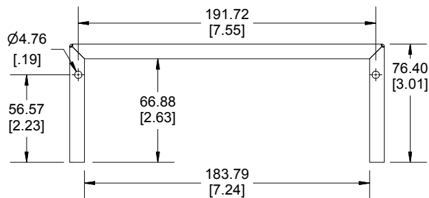
Side View of Cover
