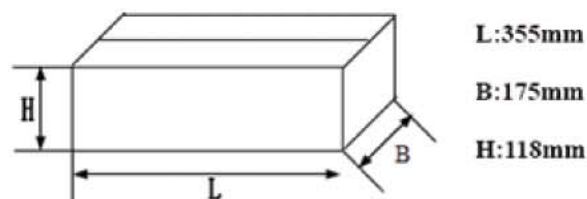
Plane drawing
