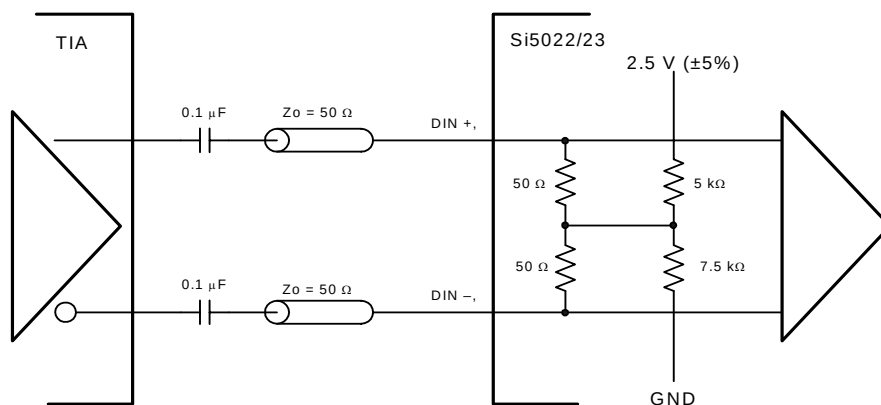
Figure 13. Input Termination for DIN (ac coupled)
