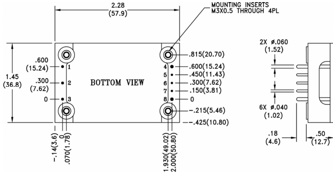
Figure 15. Mechanical Drawing
