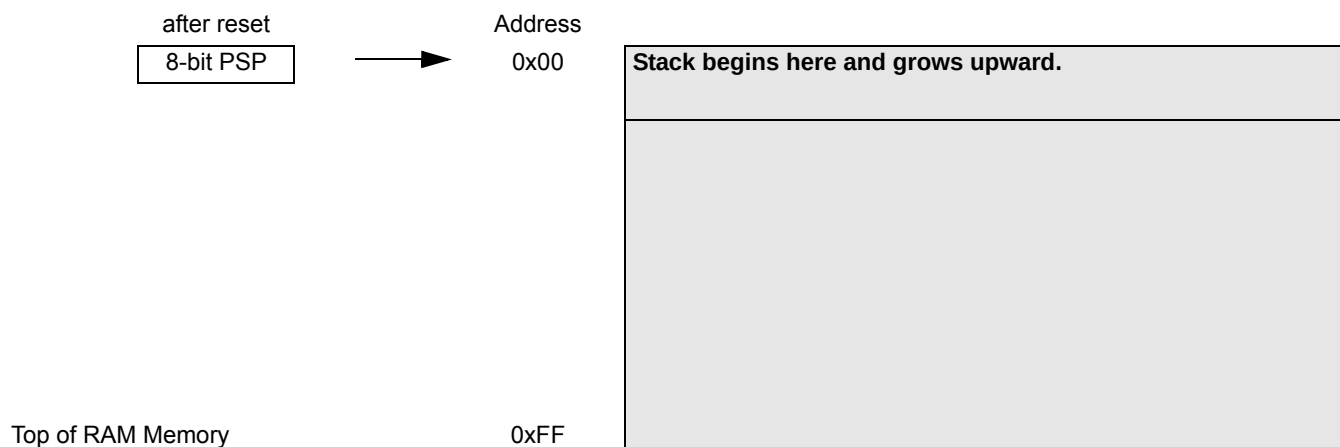
Figure 9-2. Data Memory Organization
