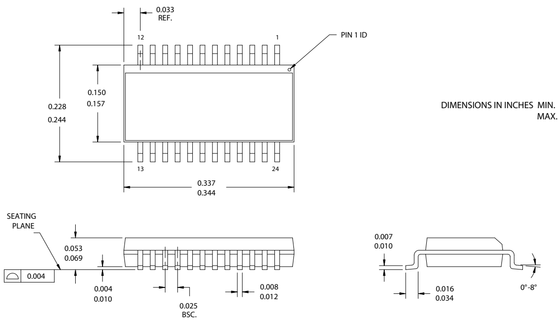
Figure 31-6. 24-Pin QSOP O241
