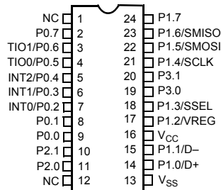
CY7C63823 24-Pin QSO
