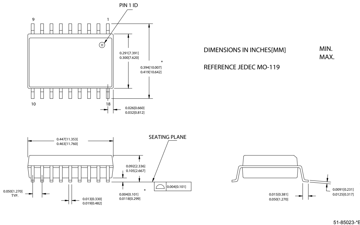
Figure 31-4. 18-Pin (300-Mil) Molded SOIC S3
