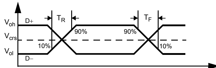
Figure 28-3. USB Data Signal Timing
