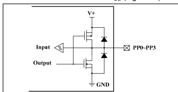
Figure 9 IS31O7328 Push-Pull I/O Ports Structure
